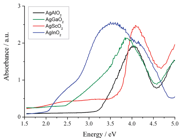
Figure 5. Kubelka-Munk absorption spectra of as-prepared silver delafossites.
