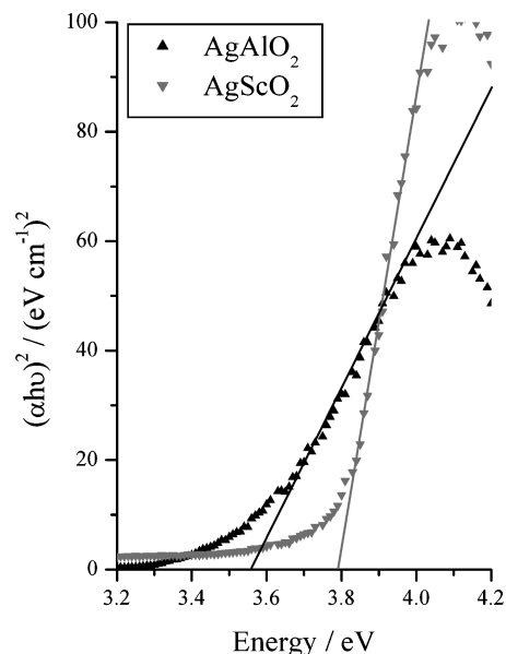
Figure 6. Plot of (\alpha h\nu)^2 versus h\nu for \text{AgAlO}_2 (black) and \text{AgScO}_2 (gray). The absorption coefficient ( \alpha ) is estimated by the Kubelka-Munk conversion of diffuse reflectance.
