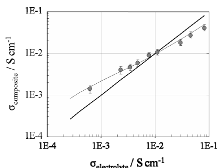
Figure 13. Plot that summarizes the PSC conductivity measurements for AgAlO 2 . The gray data points represent the measured conductivity of the PSC, while the black line represents the conductivity of the electrolyte solution. A conductivity estimate is given where the composite and electrolyte conductivities are equivalent. A Bruggeman asymmetric model considering randomly arranged spherical particles and a broad range of sizes (volume fraction \sim 0.2 – 0.3 ) was used.
