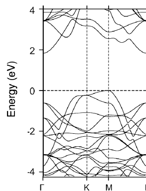
Figure 10. Calculated band structure for AgScO 2 . Energy zero is at the highest valence band at M.
