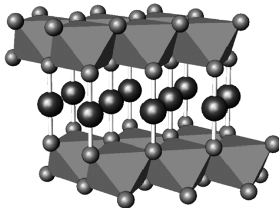
Figure 1. Schematic representation of the delafossite structure ( \text{ABO}_2 ). The gray polyhedra and black spheres represent edge-shared \text{B}^{3+}\text{O}_6 distorted octahedra and linearly coordinated \text{A}^+ cations, respectively.
