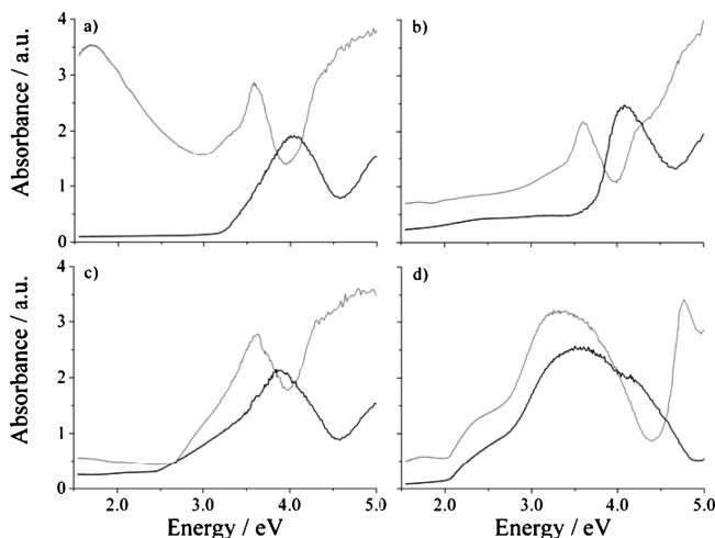
Figure 7. Kubelka-Munk absorption spectra of as-prepared silver delafossites (black lines) compared to their corresponding copper delafossites (gray lines) shown for (a) \text{AAIO}_2 , (b) \text{AScO}_2 , (c) \text{AGaO}_2 , and (d) \text{AInO}_2 .
