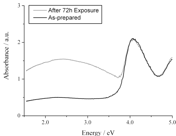
Figure 12. Kubelka–Munk absorption spectra of as-prepared AgScO 2 before and after exposure to visible light for 72 h.
