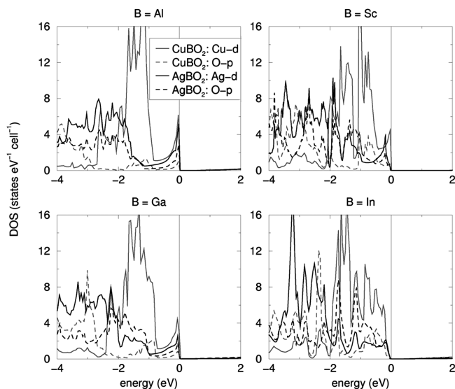
Figure 11. Projected densities of A d and O p states for (a) AAIO 2 , (b) AScO 2 , (c) AGaO 2 , and (d) AInO 2 , where A = Cu (gray lines) or Ag (black lines). In these plots, the top of the valence band is taken as zero on the energy axis.
