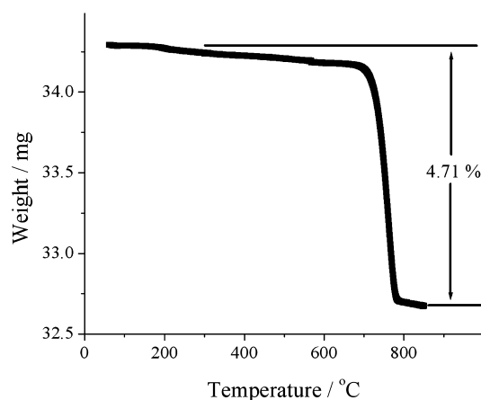
Figure 3. Plot of the TGA of \text{AgAlO}_2 reduced in a \text{N}_2 atmosphere. The final products (verified by XRD) were \text{Al}_2\text{O}_3 and silver metal.
