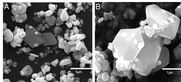
Figure 2. SEM images for (a) a mixture of \text{AgScO}_2 crystallites ranging in size from a few tenths of one micron up to \sim 5 \mu\text{m} and (b) a close-up view of some micron-sized hexagonal plates of \text{AgGaO}_2 .
