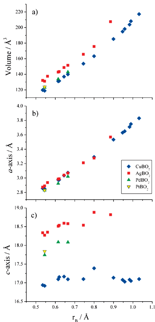
Figure 8. Graph illustrating the relationship between the ionic radius of the B-site cation and (a) the unit cell volume, (b) the a -axis length, and (c) the c -axis length for delafossites.
