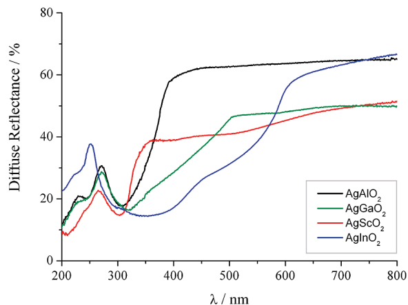
Figure 4. Diffuse-reflectance spectra of as-prepared silver delafossites.
