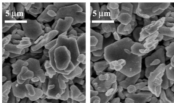
Fig. 1. SEM images of large, highly crystalline grains of \text{AgInO}_2 grown hydrothermally.
