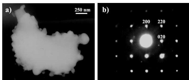
Fig. 4. Electron micrographs of (a) an image of a typical \text{Ag}_2\text{O} grain, as received from vendor, and (b) a diffraction pattern, along the [001] zone axis of Ag, as taken from a globule.
