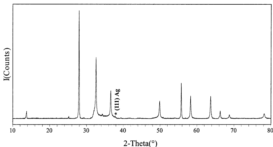
Fig. 2. Powder X-ray diffraction pattern of 3R- \text{AgInO}_2 .
