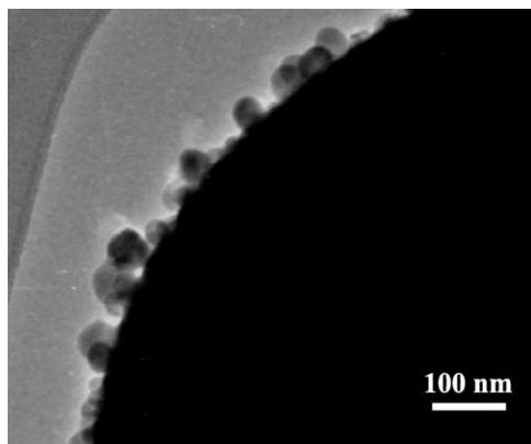
Fig. 5. TEM image of an oxidized \text{Ag}_2\text{O} particle illustrates the presence of Ag globules on the grain edge.
