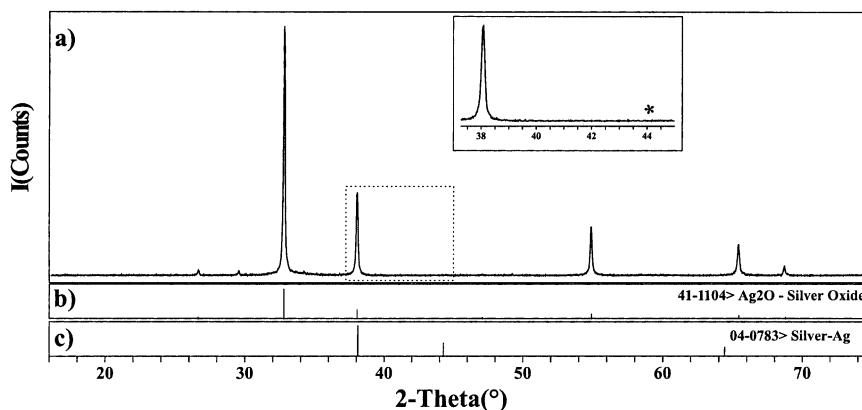
Fig. 3. (a) Powder XRD pattern for typical \text{Ag}_2\text{O} as received from vendor ( K\beta transition at 2\theta = 29.413^\circ ), with inset from 37.5 < 2\theta < 45.5^\circ illustrating location, marked by asterisk, where (200) reflection of metallic Ag would appear. Calculated positions, both indexed and showing relative intensities marked by vertical bars, of (b) \text{Ag}_2\text{O} (JCPDS #41–1104) and (c) Ag (JCPDS #04–0783).
