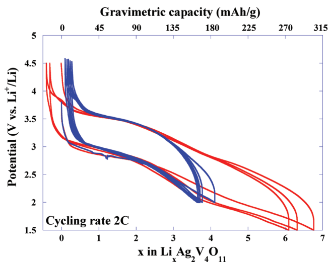
Figure 3. Galvanostatic curve recorded at 2C in the range 2–4.5 V or 1.5–4.5 V (vs \text{Li}^+/\text{Li} ) of a composite SVO-RT/ \text{C}_{\text{sp}} electrode in 1 M \text{LiPF}_6 EC/DMC 1:1 electrolyte.
